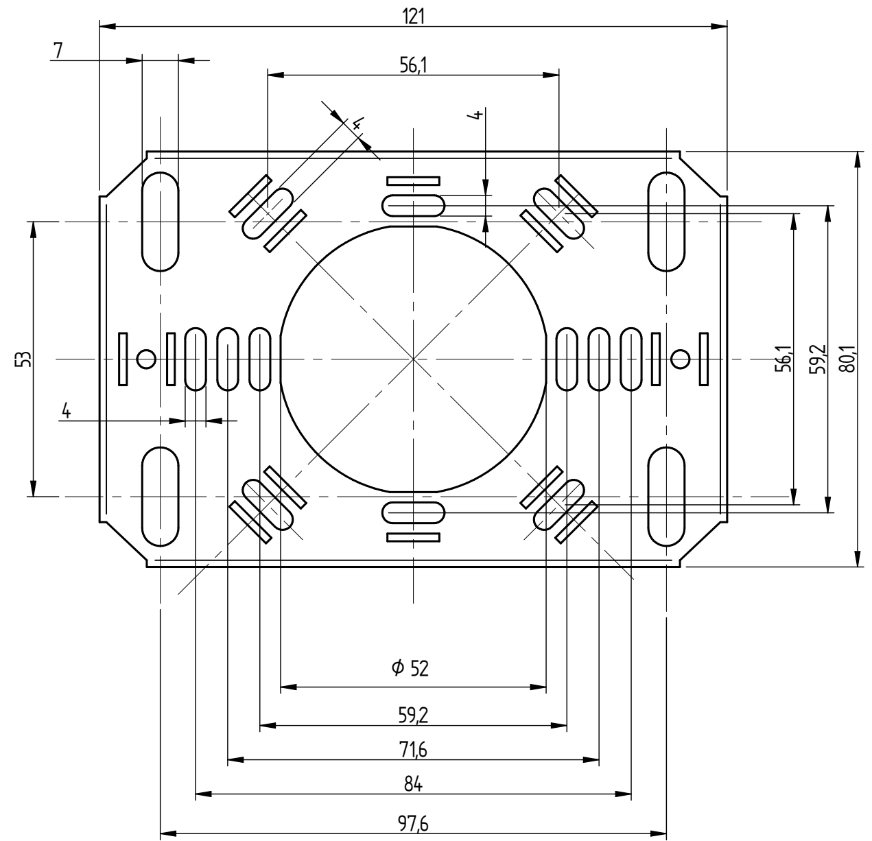
MOUNTING BRACKET
